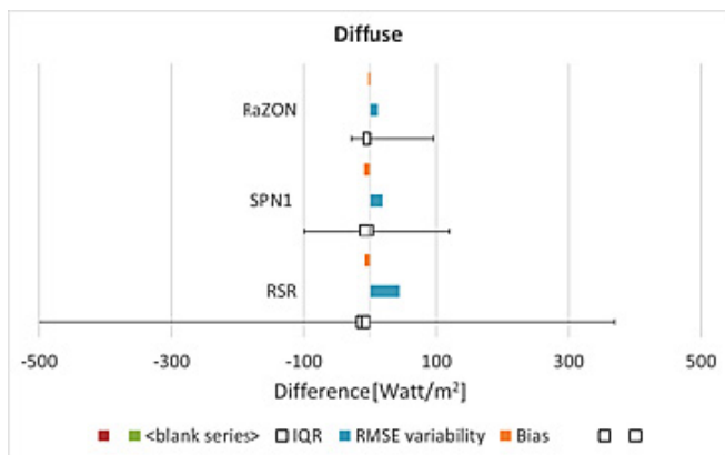
Figure 9 The same analysis as in figure 8 for the DHI.
