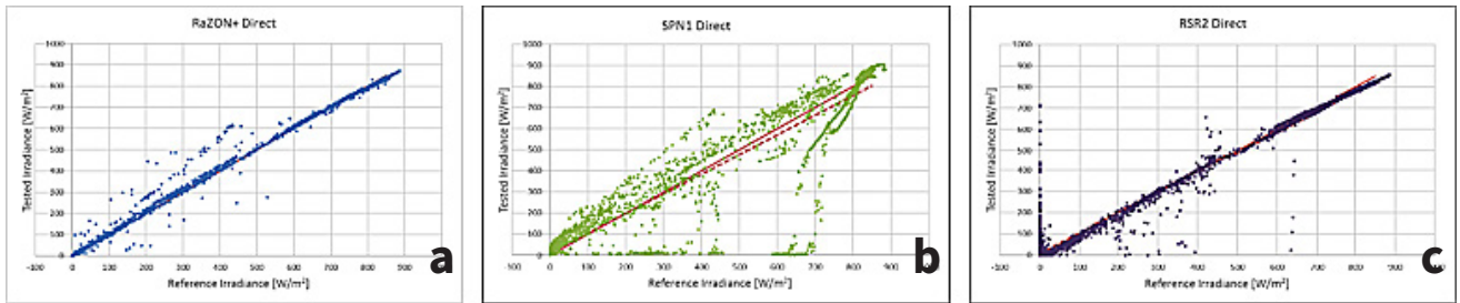
Figure 5 DNI measurements plotted with on the x-axis the reference irradiance and on the y-axis the (a) RaZON + , (b) SPN1, and (c) RSR2 data. The solid red line is y=x and the dashed red line is the fit of the measurement points.
