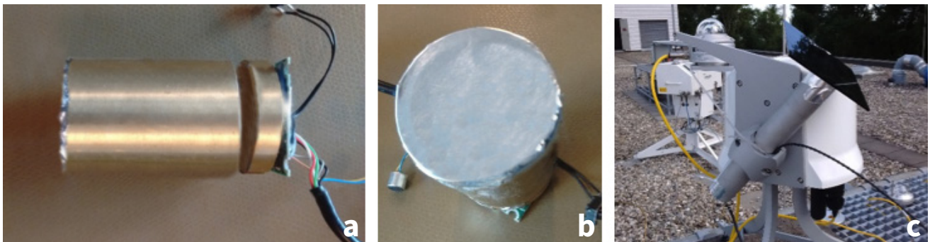
Figure 2 (a) Pointing accuracy apparatus consisting of a brass tube with a pinhole in aluminium at the left and a CMOS camera at the right end, (b) aluminium foil with pinhole, and (c) the pointing accuracy apparatus on the RaZON + .
