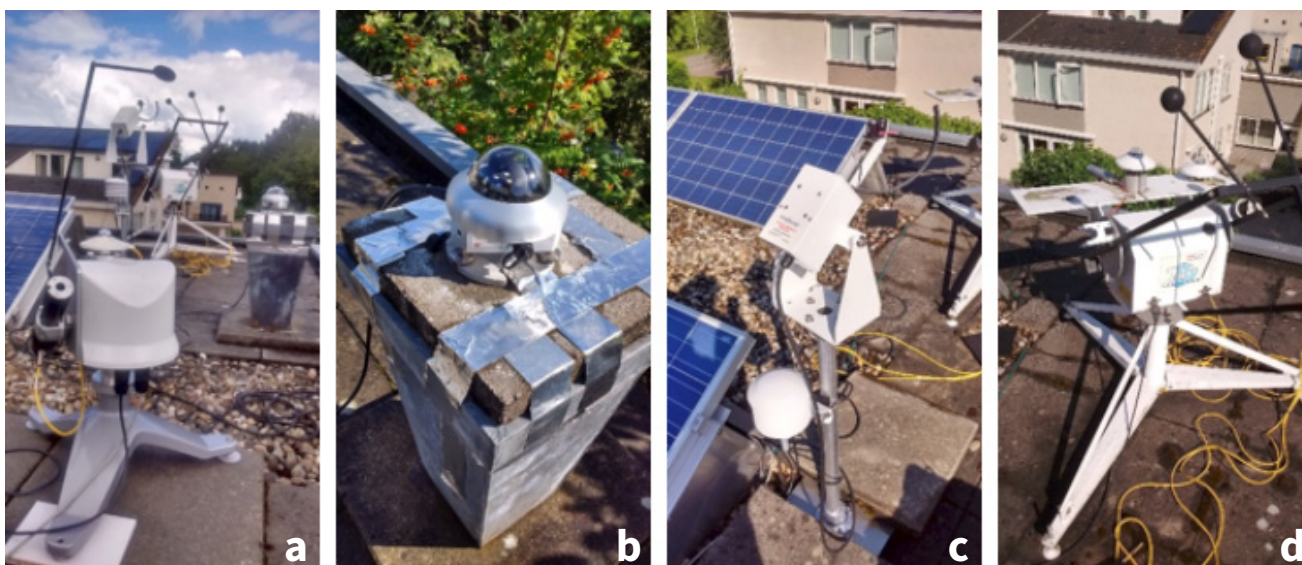
Figure 3 rooftop setup (a) all the solar monitoring systems (b) SPN1 Sunshine Pyranometer, (c) RSR2 Rotating Shadowband Radiometer, and (d) Kipp & Zonen reference station.
