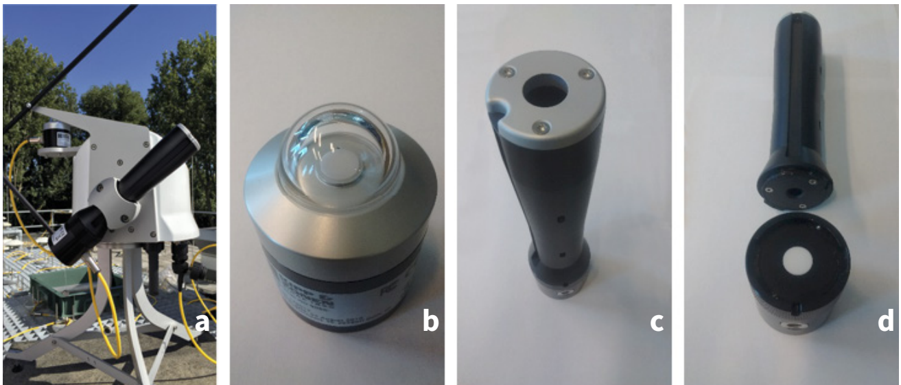
Figure 1 (a) The RaZON + at the measurement location, (b) the RaZON + PR1 pyranometer, (c) PH1 pyrhelimeter, and (d) PH1 collimation tube separate from detector unit.
