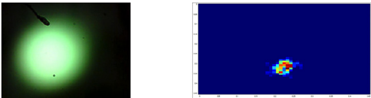
Figure 4 (a) the image of the sun on the camera in the pointing accuracy apparatus, and (b) a pointing angle density plot over 2200 image frames of the sun projection centre. The pointing angle density plot has the angle on the x and y axis; The colour map from red to yellow to light blue and dark blue denotes a high frequency to a low frequency of the pointed angle.
