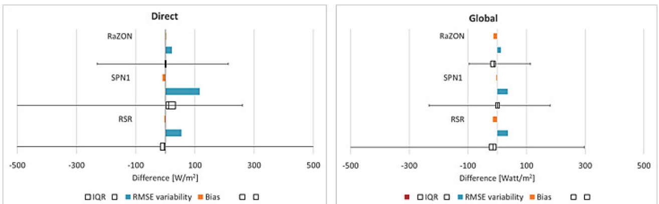
Figure 8 For the difference of the RaZON + , SPN1 and RSR2 and the reference the bias, RMSE due to variability and box and whisker analysis showing the maximum and minimum (whiskers) and the 2 quartiles around the median (box) are shown. For (a) the DNI and (b) the GHI.
