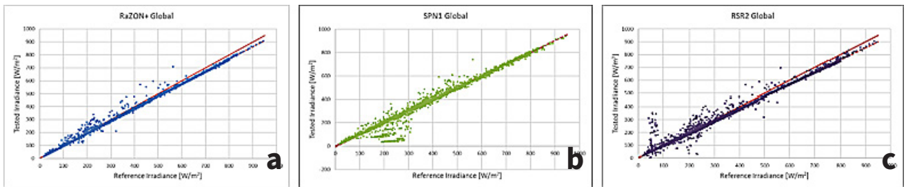
Figure 6 GHI measurements plotted with on the x-axis the reference irradiance and on the y-axis the (a) RaZON + , (b) SPN1, and (c) RSR2 data. The solid red line is y=x and the dashed red line is the fit of the measurement points.
